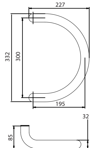
D Handle
