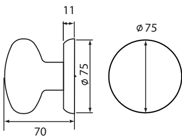
Centre Knob
