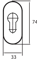
Oval Escutcheon
