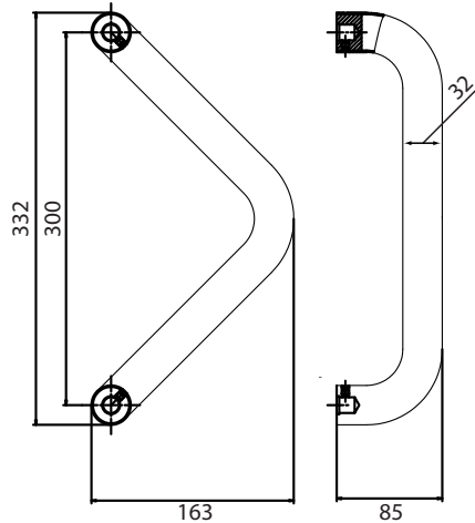
V Handle
