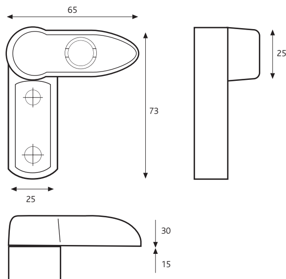
Keyless Snaplock
