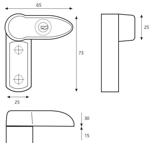
Keyed Snaplock
