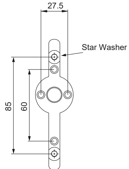
Fixing Bracket
