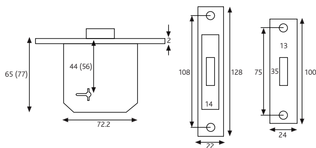
3 Lever Deadlock
