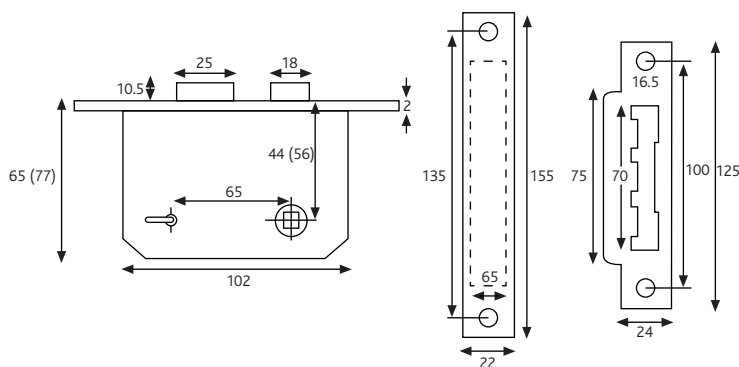
3 Lever Sashlock
