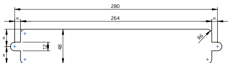
Routing Detail
